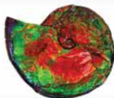
Canadian Ammonites
